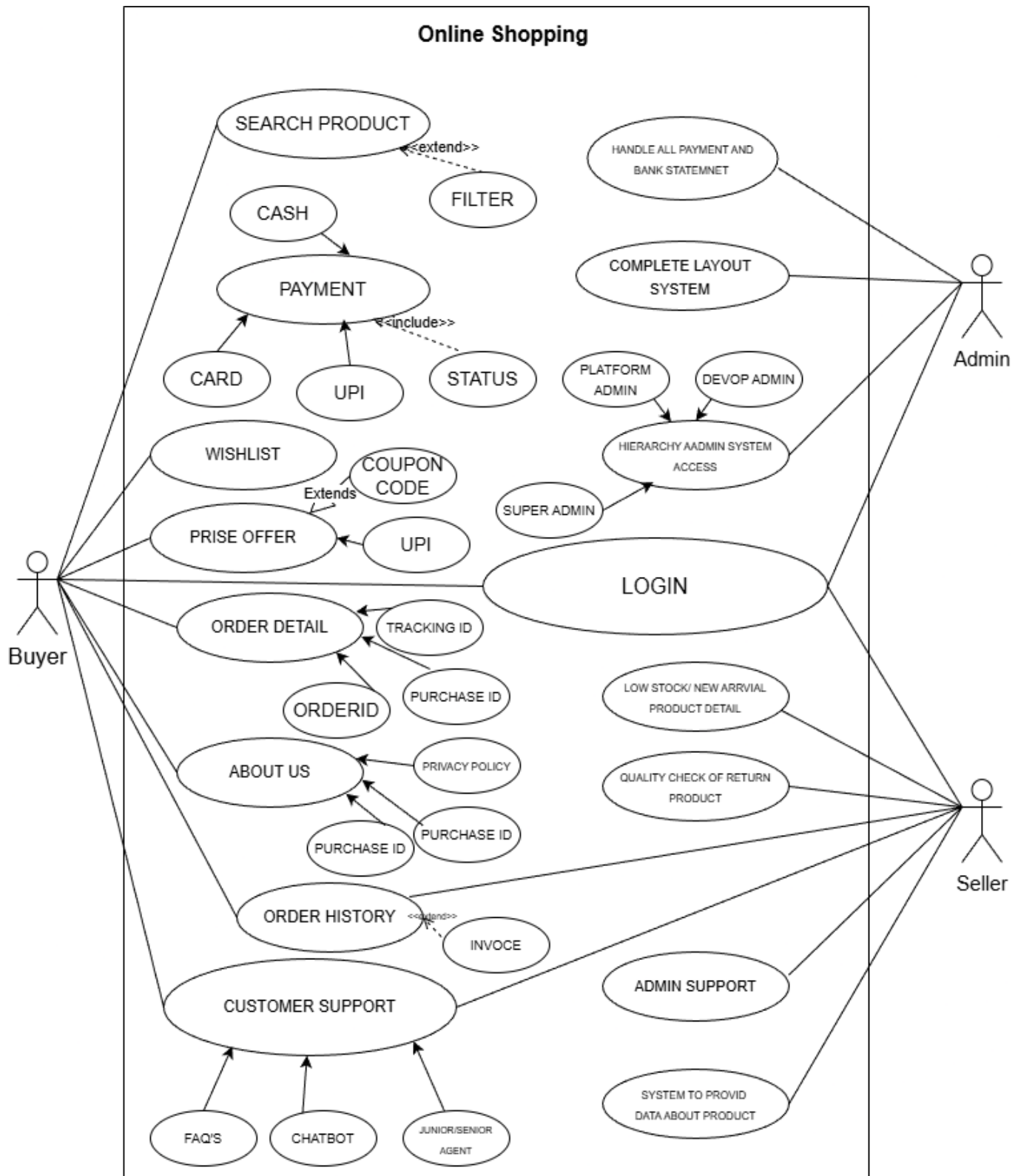
Figure 2.1-1 Use case diagram for Online Shopping system
